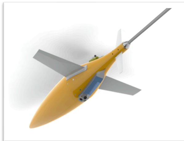
Figure 4. Drawing of a 1 MHz Nortek Profiler for the Seaglider. The full package, including the 4-beam transducer head, profiler electronics, tilt sensor, compass and internal memory, is mounted in a low-profile anodized aluminum housing rated for 1000 m.
