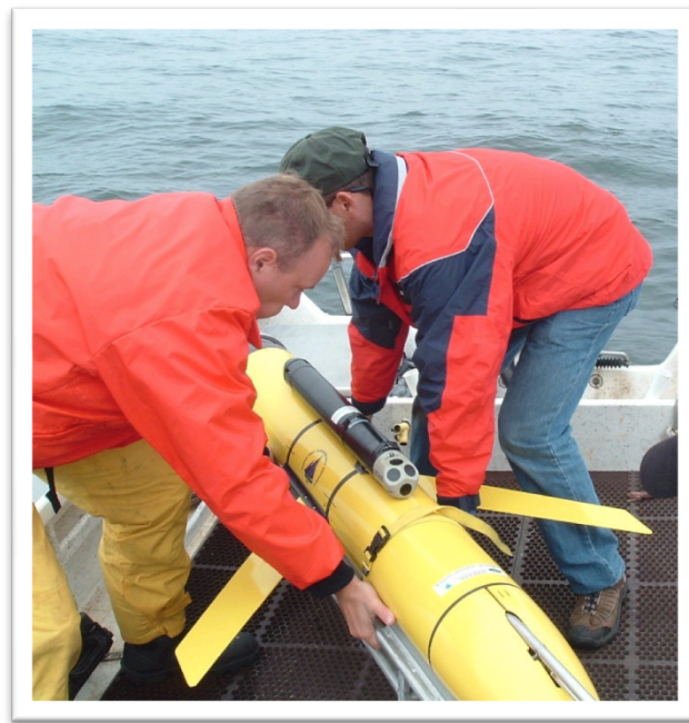
Figure 1. Deployment of a Webb Slocum 200 m glider with self-contained Nortek 1 MHz Aquadopp Profiler. A fleet of similarly-equipped vehicles were used by WHOI researchers to explore relationships between physical and biological fine structure in the ocean.
