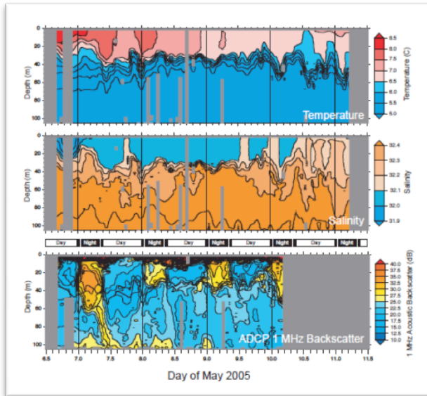
Figure 2. Time series of temperature, salinity, and backscatter amplitude collected during May 2005 in the Great South Channel east of Cape Cod, MA. Acoustic backscatter at 1 MHz has been shown to be an effective proxy for the vertically-migrating copepod Calanus finmarchicus .
