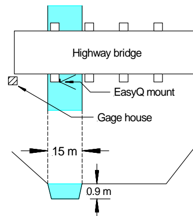
Figure 6. Sketch of the Fall Creek deployment site
