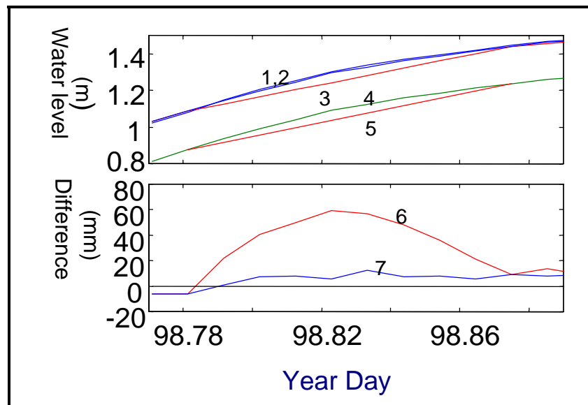
Figure 9. Interpolation of stage data. (1,2) EasyQ corrected stage and shaft encoder stage. (3) EasyQ stage corrected with only linear interpolation. (4) EasyQ pressure. (5) Linearly interpolated pressure, using the same endpoints as used for trace 3. (6) Difference between shaft encoder stage and trace 3. (7) Difference between final corrected stage and shaft encoder stage.
