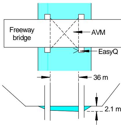
Figure 5. Plan view of White River installation site.
