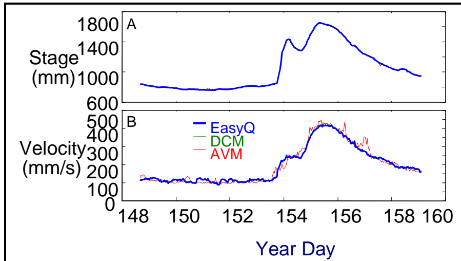
Figure 7A. Stage measured by EasyQ (heavy line) and AVM (thin line). The AVM line is barely visible behind the EasyQ line. Day 148 corresponds to May 27, 1999.
