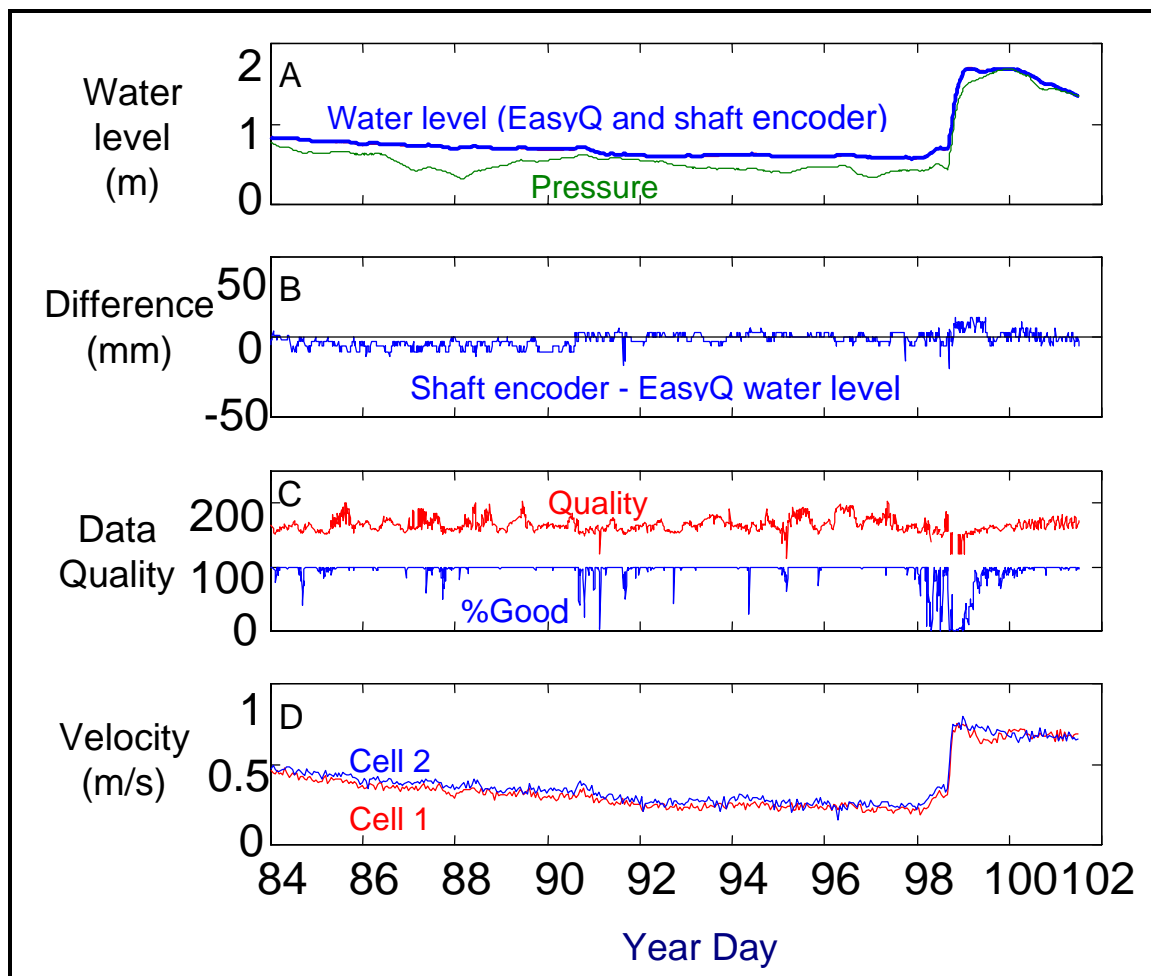
Figure 8. Water level measured by EasyQ and shaft encoder (A), difference between shaft encoder and EasyQ (B), the EasyQ stage quality and % good parameters (C), and the measured velocities in cell 1 and 2 (D). Day 84 corresponds to March 24, 2000.
