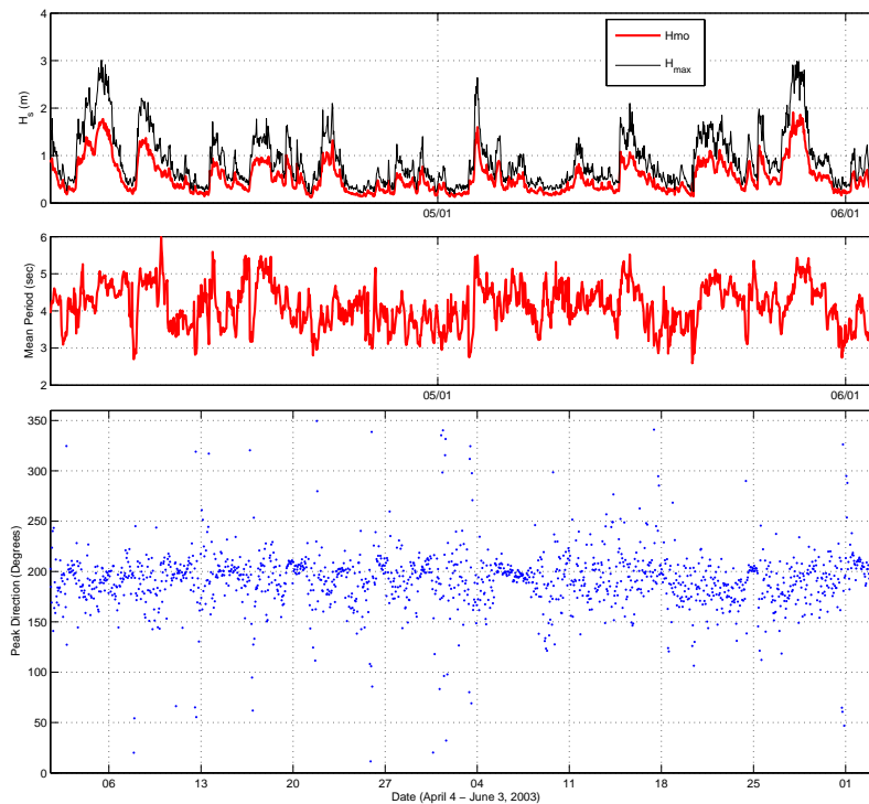
Figure 5 Wave burst estimates for Malaga, Spain: (A) upper plot is H_{m0} (thick line) and H_{max} (thin line) (B) the middle plot is the mean period, (C) Example of the Peak direction based upon the first pair of Fourier coefficients, which gives an misleading direction.
