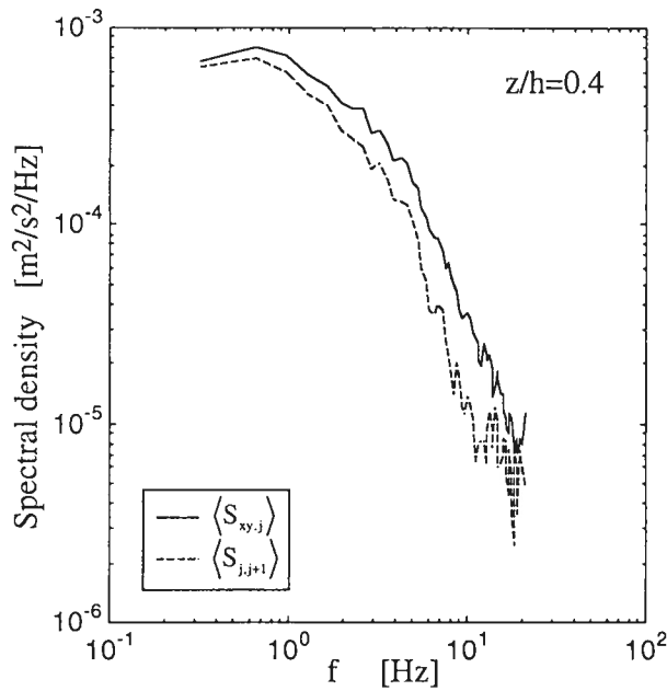
FIG. 7. Spectra of the vertical fluctuating velocity component at depth z/h = 0.4 . The solid line represents the result of the cross-correlation between the measurements in the longitudinal and transverse flow sections. The dashed line shows the result of the cross-correlation between two consecutive points as proposed by Garbini et al. (1982).
